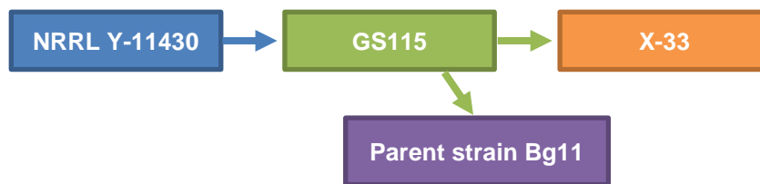
Figure 1: Lineage of the Pichia pastoris host organism Bg11. NRRL Y-11430 is the one of the original isolates from which many of the commercialised P. pastoris strains such as GS115 (Cregg et al. 1985), were derived for the production of food and industrial chemicals.
